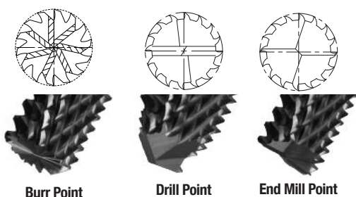
Burr Point
